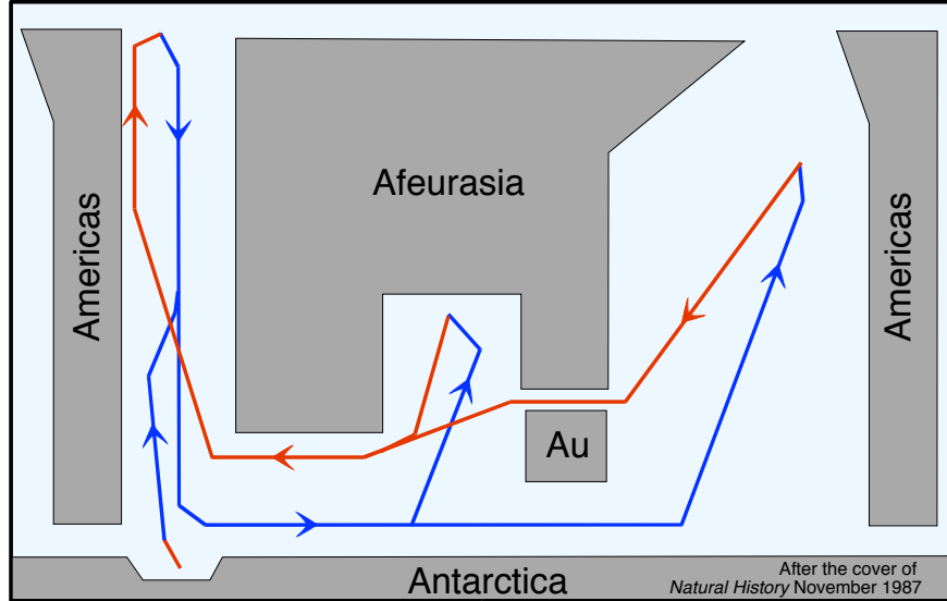
A. Broecker's Great Ocean Conveyor, as commonly portrayed
