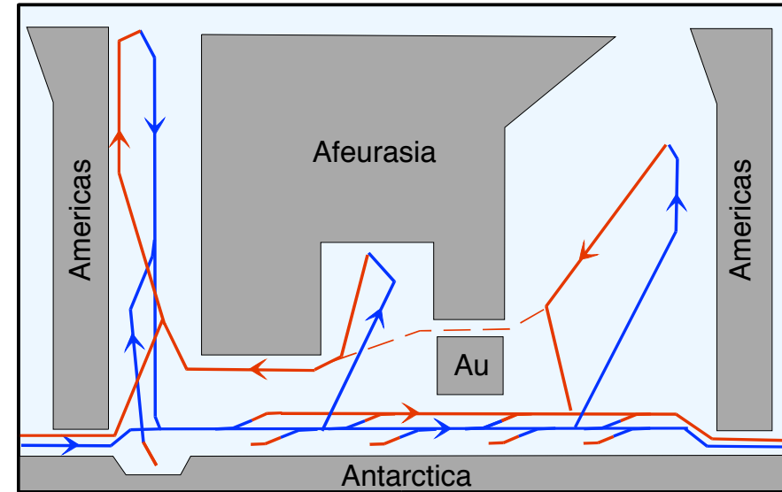
D. A synthesis of B and C
