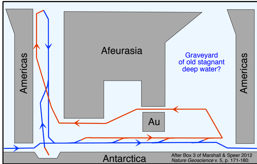
C. Antarctic Upwelling model in Box 3 of Marshall and Speer (2012)
