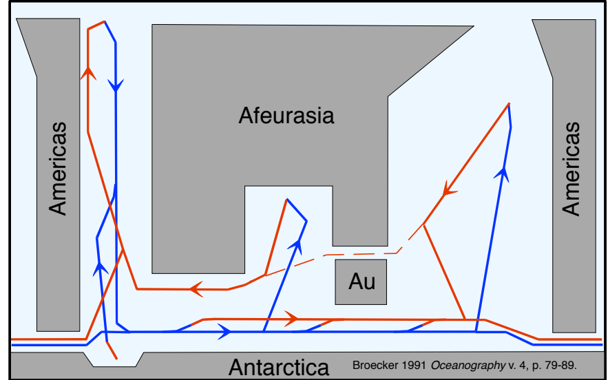
B. Broecker's Great Ocean Conveyor, as described in Broecker (1991)
